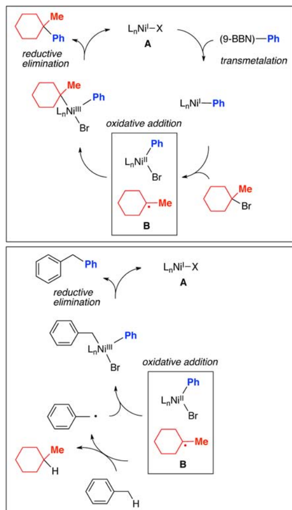
Figure 1. (top) Outline of a possible mechanism for the Ni/I-catalyzed Suzuki cross-coupling of an unactivated tertiary alkyl bromide. (bottom) Possible pathway for the formation of diphenylmethane when toluene is employed as the solvent (the early steps of the catalytic cycle are as illustrated at the top and have been omitted for simplicity).
